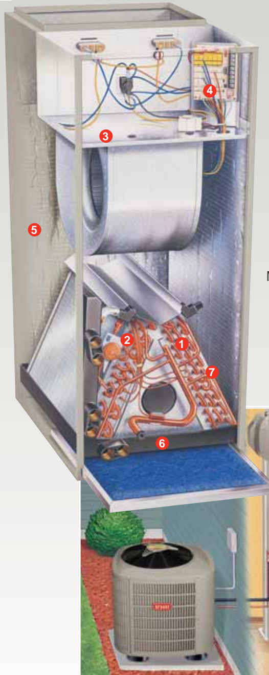
Heat Pump and Fan Coil System
